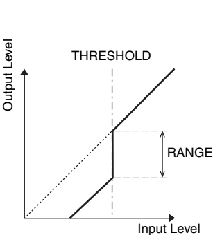
I/O Characteristics
