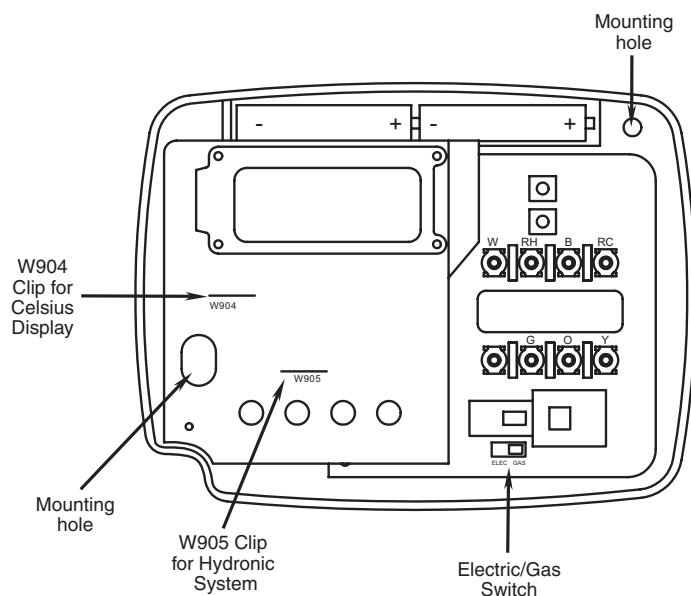
Figure 1. Thermostat
