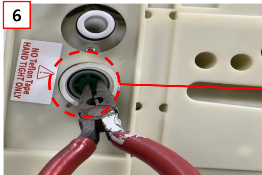
⑥ Use a tool to hold the groove of the water pressure regulator.
