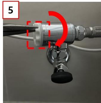
⑤ Reattach the strainer by turning it in the direction of the arrow using a tool.
