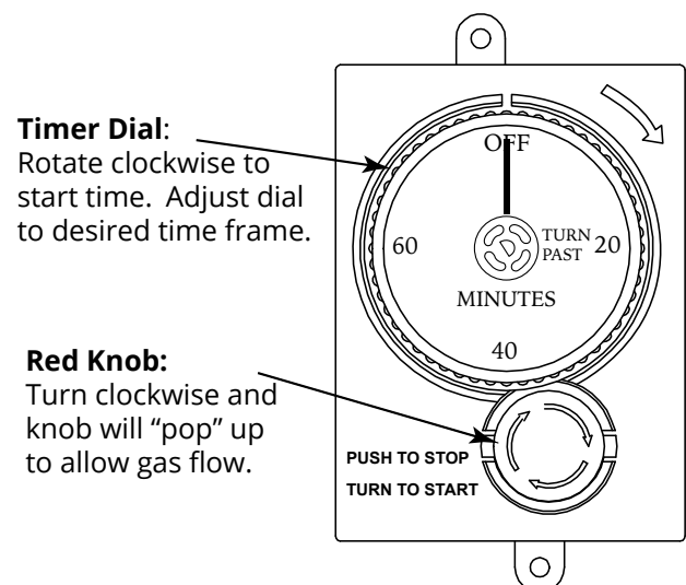
Fig. 4 E-Stop operation.
