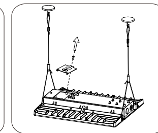
3. Remove the screws and remove the cover
