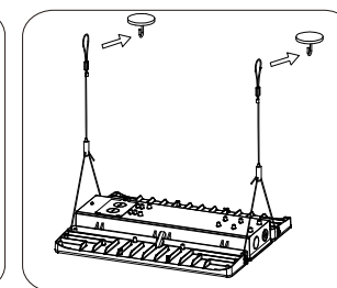
2. Hang the lanyard from the ceiling anchor
