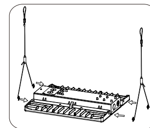
1. Install the lanyard into the light fixture
