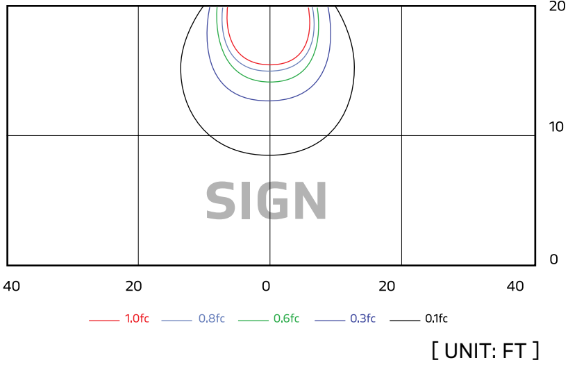
BROADWAY 10W [ MOUNTING HEIGH: 20FT ]
