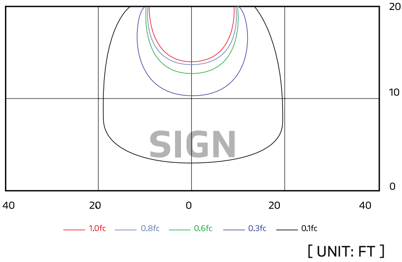
BROADWAY 20W [ MOUNTING HEIGH: 20FT ]
