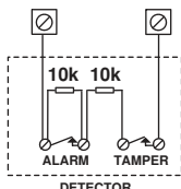
DOUBLE END OF LINE INPUT CONFIGURATION
