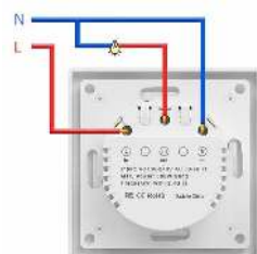
CONNECTION DIAGRAM
