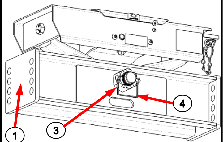
REAR VIEW OF 5 TH WHEEL HITCH
