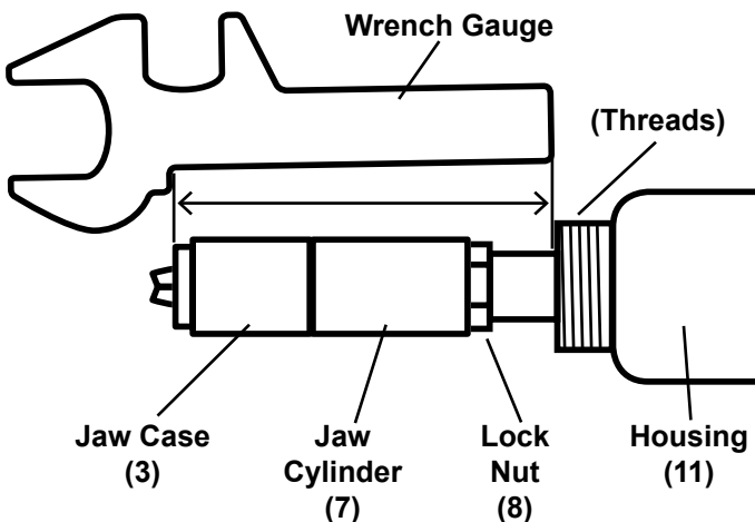
Figure D: Checking Jaw Case Tightness
