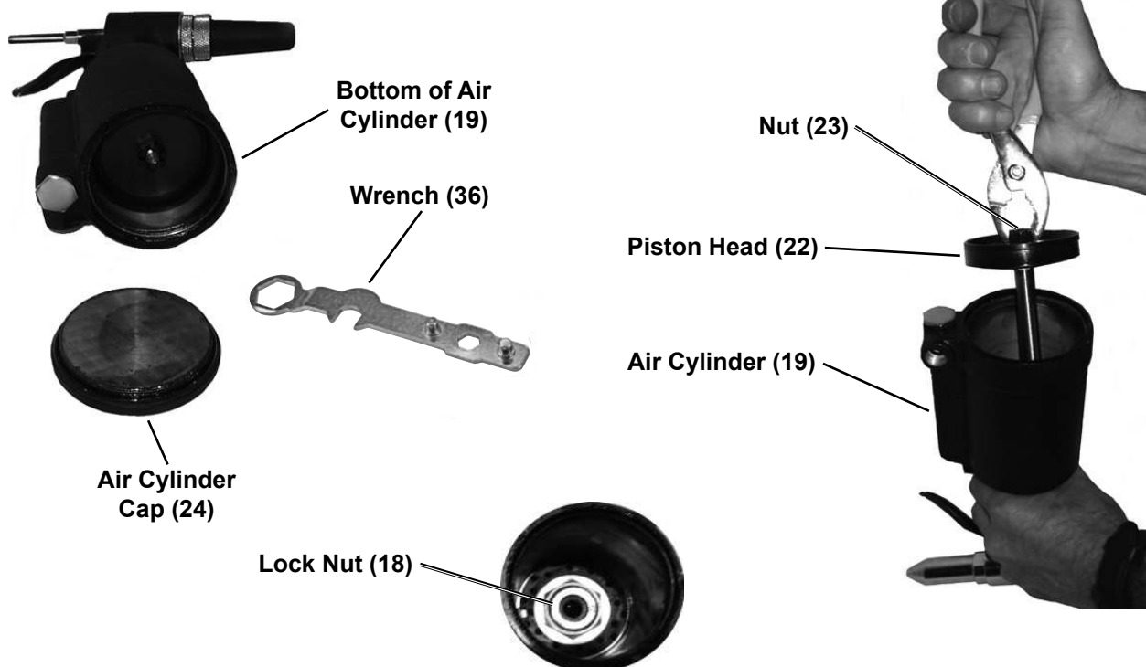
Figure C: Priming the Cylinder
