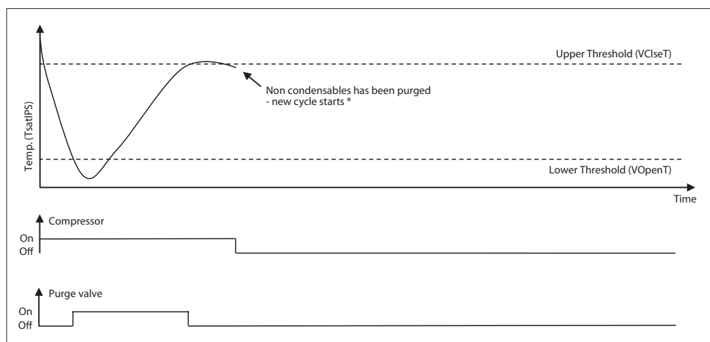
Fig. 3 - Purging procedure - Low R290 evap. temperature detected during PDT: Thresholds are configurable * If low evaporator temperature is detected (passing lower threshold), the purging procedure will be repeated immediately
