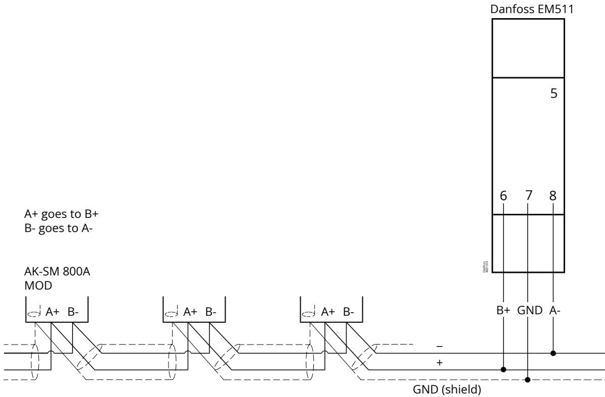
Figure: Modbus
