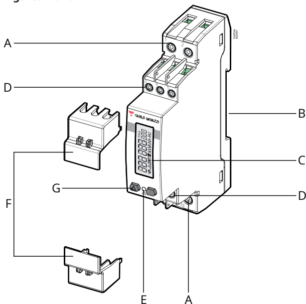
Figure: Front
